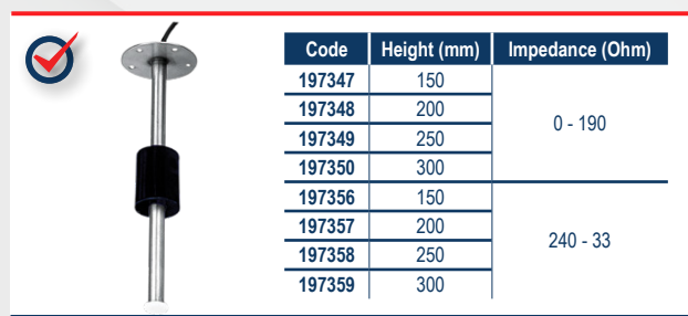
Sensor for Water Tank (12/24V, Inox 316, SAE5)
