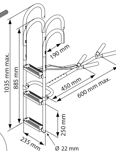
29392 Bow Ladder, Inox 316, 3 steps
