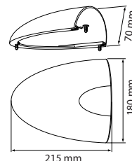
54386 Ventilation Clam Shell Cover For additional protection against heavy water intrusions. Suitable for 3" and 4" ventilators. To be fixed on top of the ventilator with 3 nylon fasteners. Made from polyamid, shock and UV-resistant. Compatible with common sealants and impervious to acetic acids. (215x180x70 mm)
