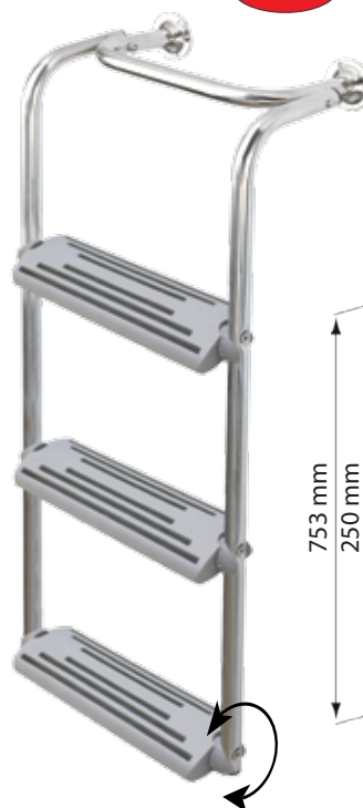
55694 Bow Ladder, Inox 316 3 steps
