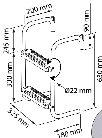
55706 Raft Ladder, Inox 316 2 steps
