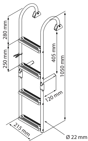
30535 Folttable Ladder, Inox 316 for Narrow Transom, 2+2 steps, 180°
